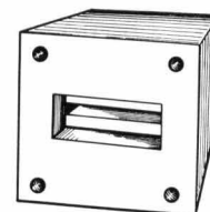
Fig. 2. Special iris used in measuring small losses consists of a thick iris with quarter wave sections on each side. Dimensions for height of slot are given in text.
